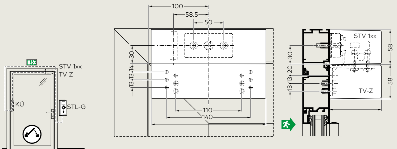
Installation on flush-mounted doors via TV-Z on the outer door, without restriction of the clear passage height, opening outwards
