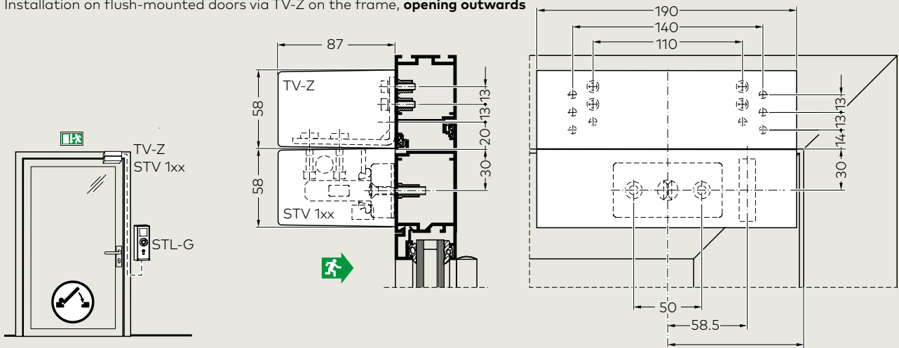
Installation on flush-mounted doors via TV-Z on the frame, opening outwards
